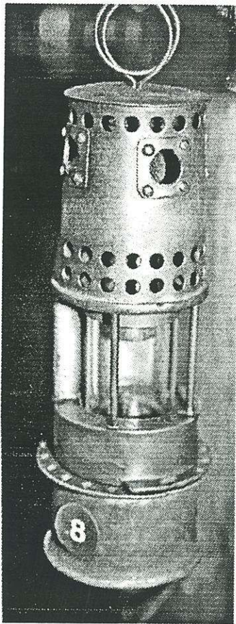
fumat lamp with Mueseler chimney, produced by Fabrique Liegeoise de Lampes de Securite, Liege, Belgium, 1905.
