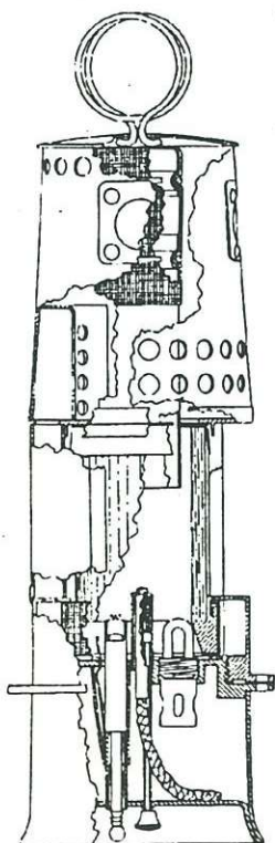
fumat lamp with Mueseler chimney, produced by Fabrique Liegeoise de Lampes de Securite, Liege, Belgium, 1905.
